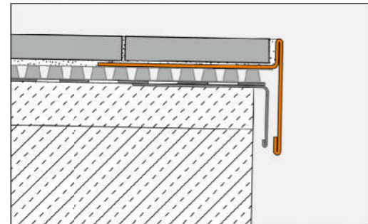
Schlüter®-BARA-RT
