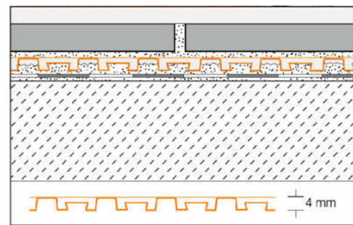
Schlüter®-DITRA-DRAIN 4
